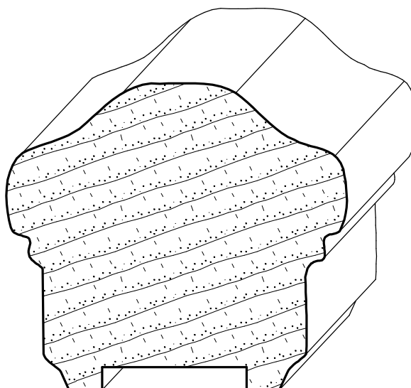
IH-714 2-1/2" x 2-1/4"
