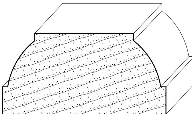
IH-730 3" x 1-1/2"
