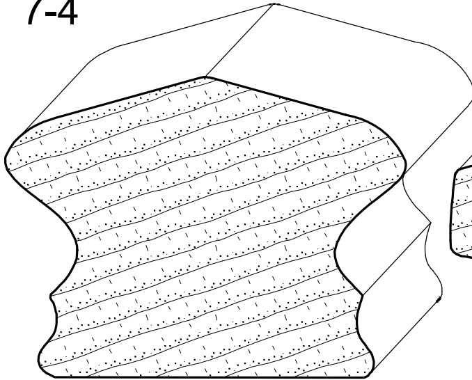
IH-712 3" x 2-1/4"
