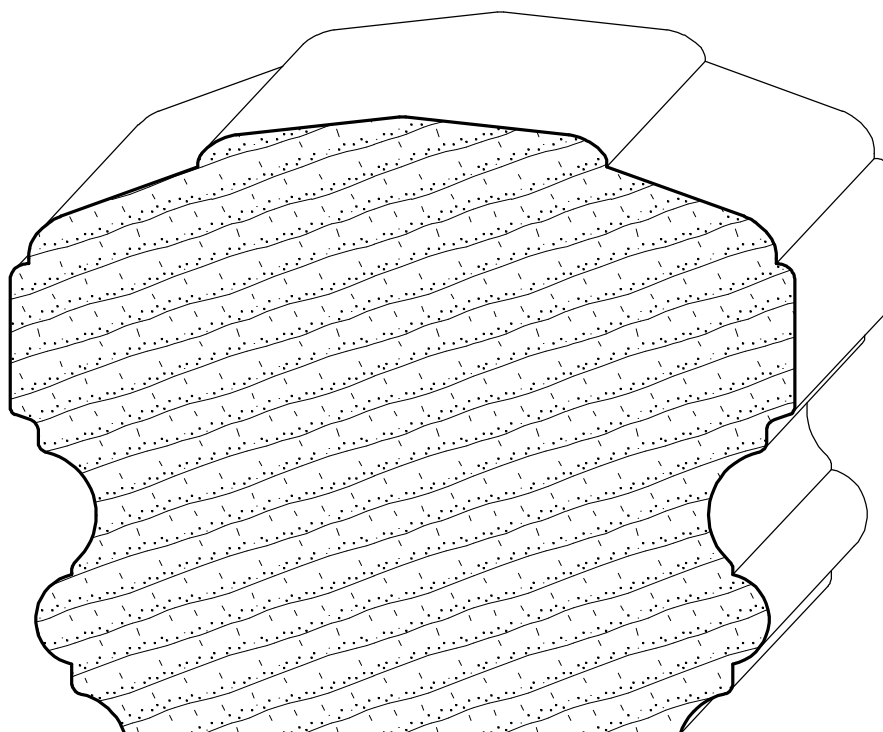
IH-720 4-1/8" x 3-1/4"
