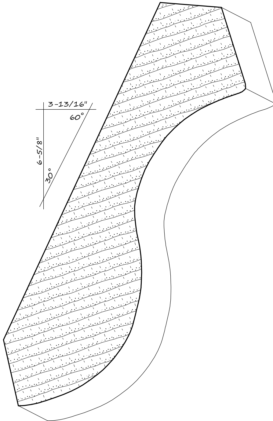
IH-671 1-15/16" x 7-5/8"
