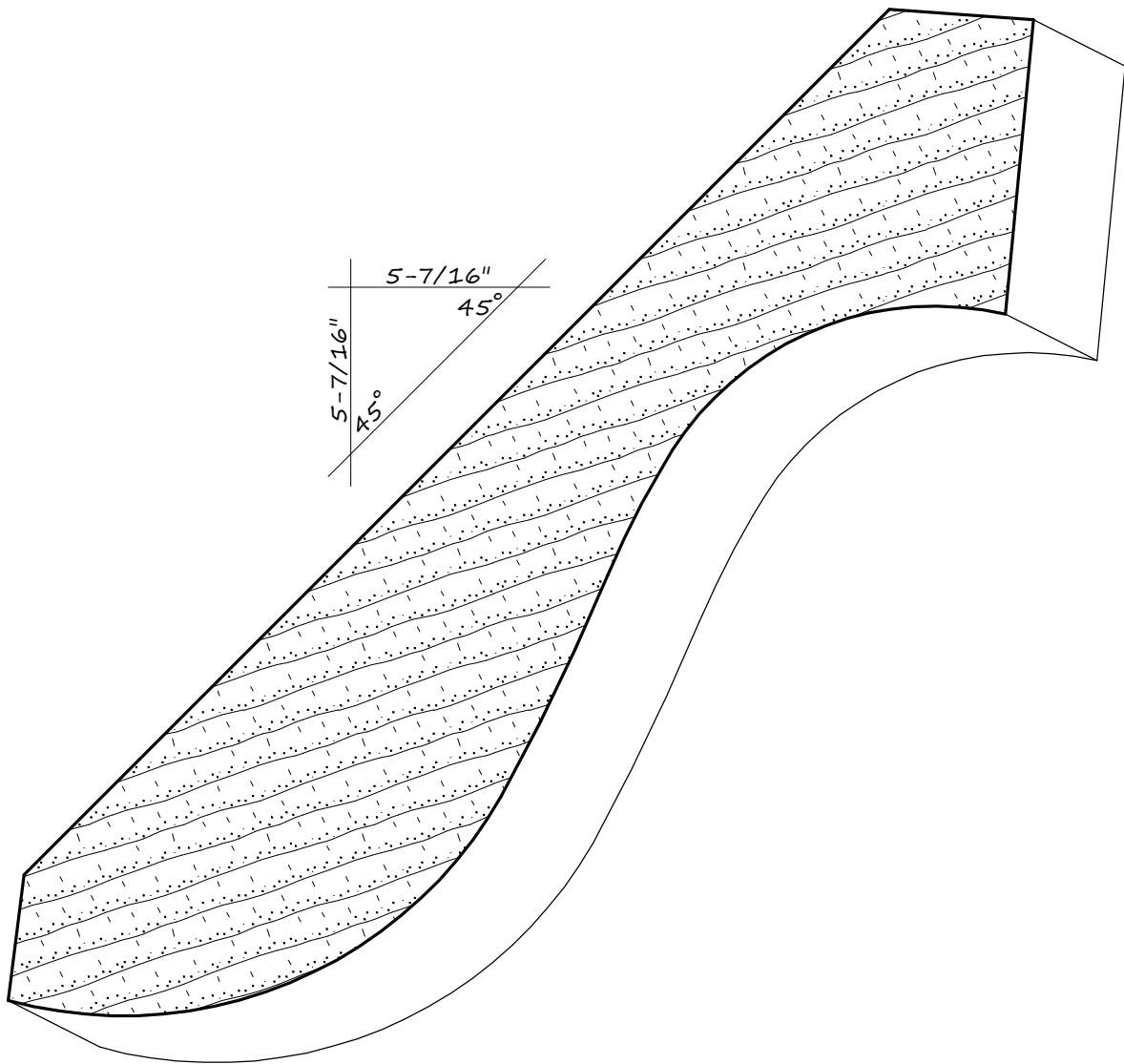
IH-1608 1-5/8" x 7-11/16"
