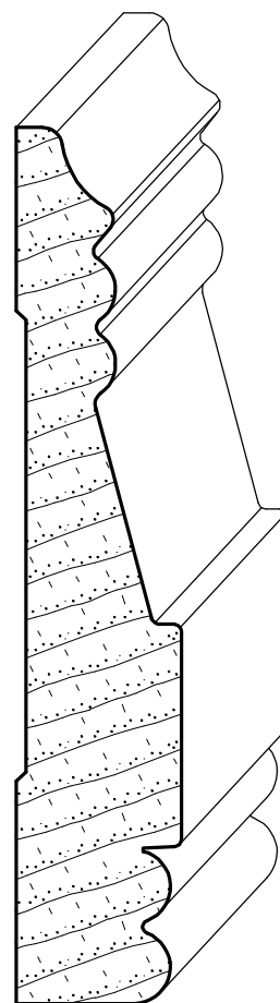
IH-1556 3/4" x 4-3/16"
