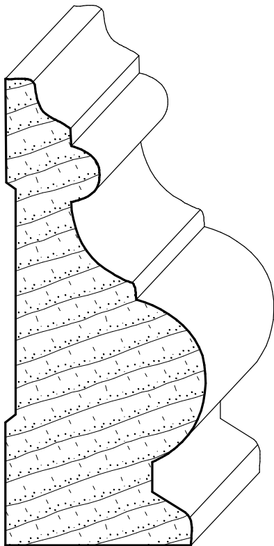
IH-593 1-1/2" x 3-1/2"
