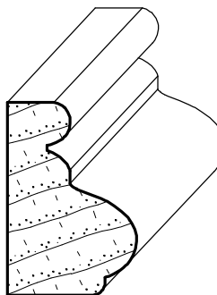
IH-590 3/4" x 1-1/8"
