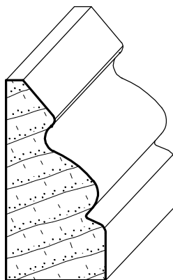
IH-584 3/4" x 1-9/16"
