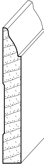
IH-582 3/8" x 2-3/4"
