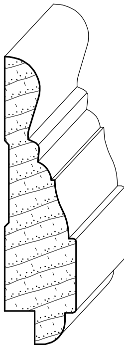
IH-1539 3/4" x 3"
