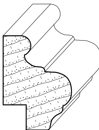
IH-535 1-3/16" x 1-5/8"
