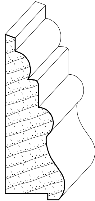
IH-587 1" x 2-3/4"
