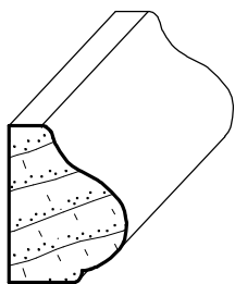
IH-536 9/16" x 3/4"
