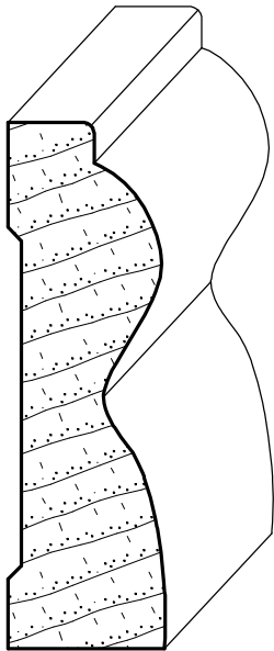
IH-595 3/4" x 2-1/2"
