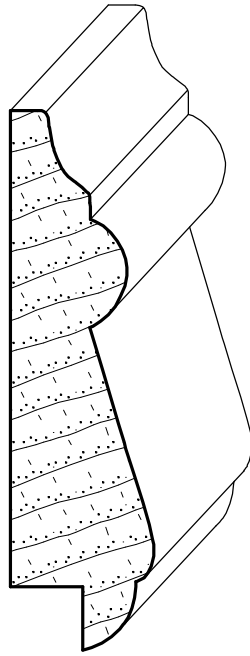
IH-551 3/4" x 2-13/16"
