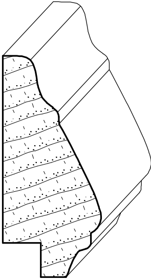
IH-519 1" x 2-1/4"
