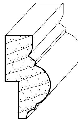
IH-567 3/4" x 1-5/16"
