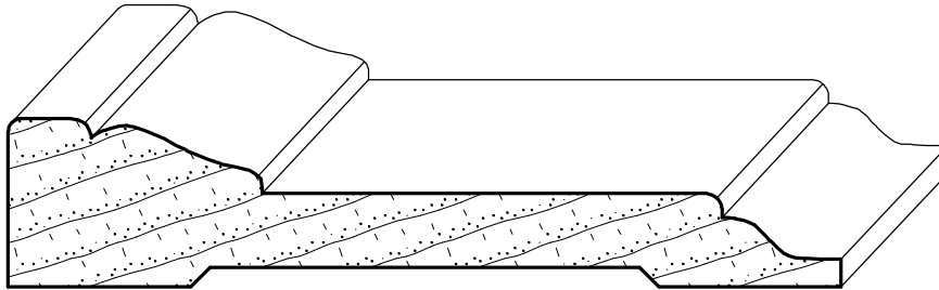
IH-1423 13/16" x 4"
