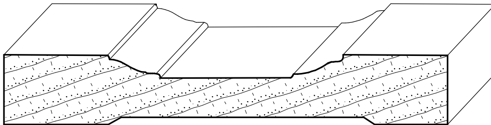
IH-480 3/4" x 4-3/4"
