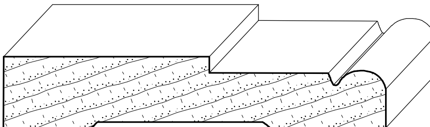
IH-429 3/4" x 4"
