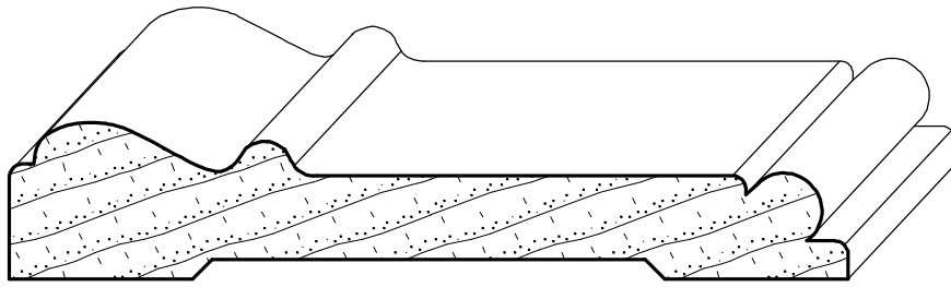
IH-1443 3/4" x 4"
