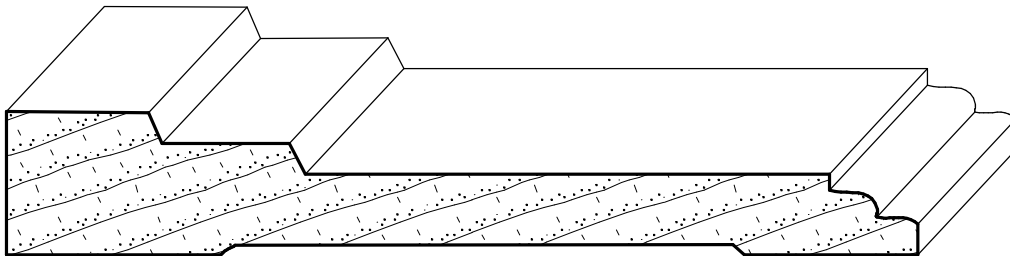
IH-441 3/4" x 4-3/4"
