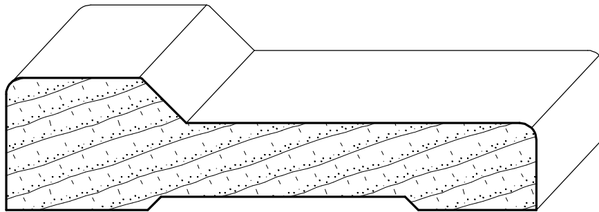
IH-1484 1" x 4"
