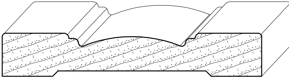
IH-1408 3/4" x 4-1/2"
