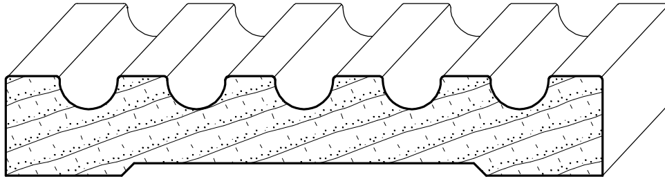
IH-1419 3/4" x 4-1/2"
