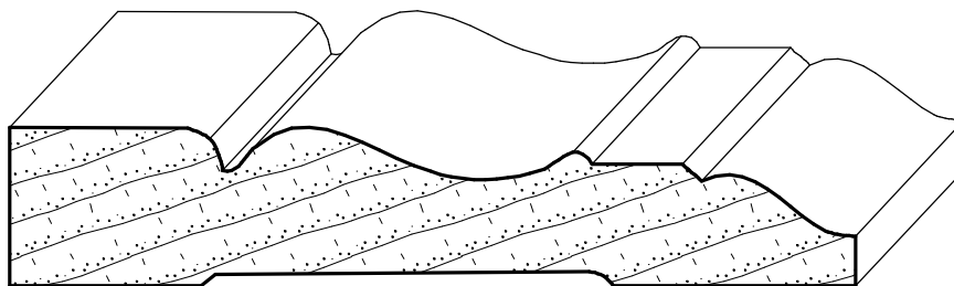
IH-464 3/4" x 4"
