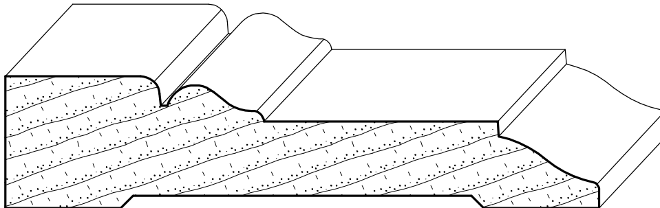
IH-447 1" x 4-1/2"
