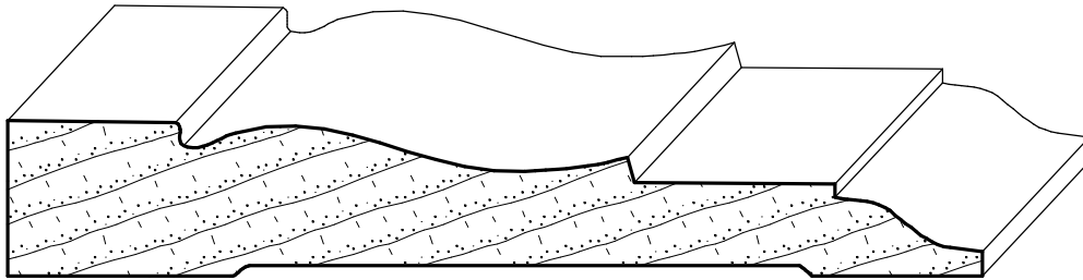
IH-408 3/4" x 4-9/16"
