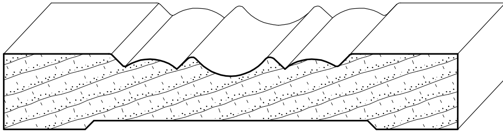
IH-1483 13/16" x 4-7/8"
