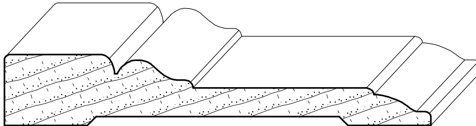
IH-1425 3/4" x 4-1/2"
