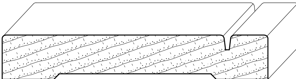
IH-1442 3/4" x 4-1/2"
