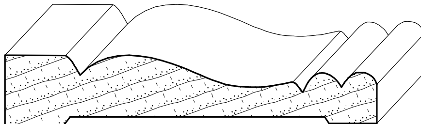
IH-481 3/4" x 4"
