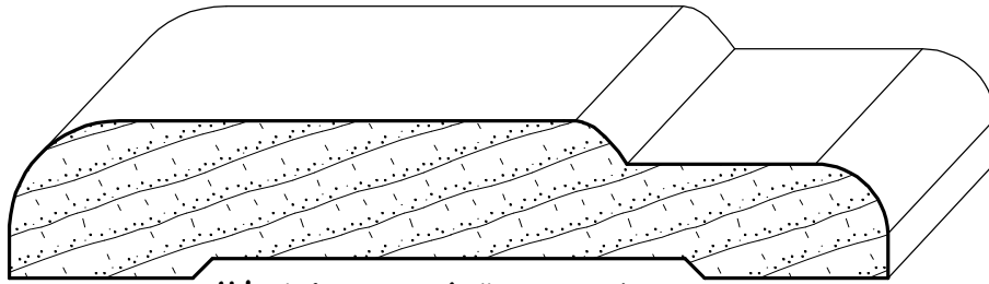
IH-1407 3/4" x 4-3/16"
