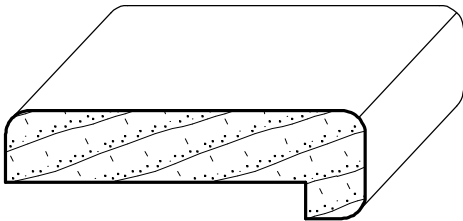
IH-142 9/16" x 1-7/8"
