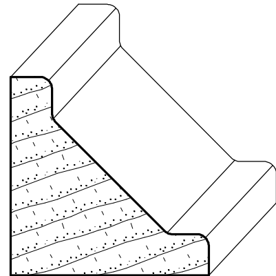
IH-159 1-1/2" x 1-1/2"
