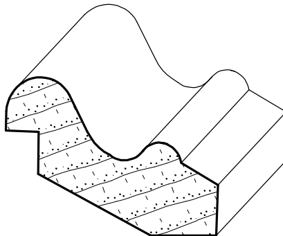
IH-158 11/16" x 1-7/8"
