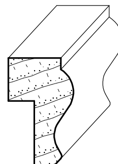
IH-1053 11/16" x 1-1/8"
