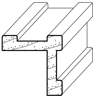
IH-193 1" x 1"
