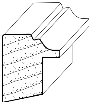
IH-162 1" x 1-3/16"
