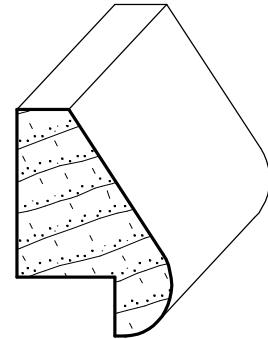
IH-144 13/16" x 1-3/16"
