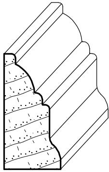
IH-133 1/2" x 3/4"
