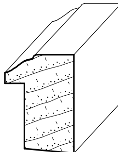
IH-1017 3/4" x 1-1/16"
