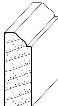
IH-1018 1/2" x 1-3/8"
